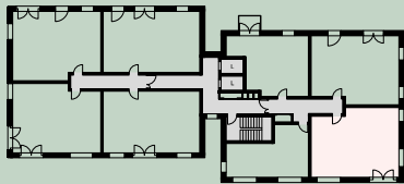
1ST - 5TH FLOOR (1ST FLOOR ILLUSTRATED)
